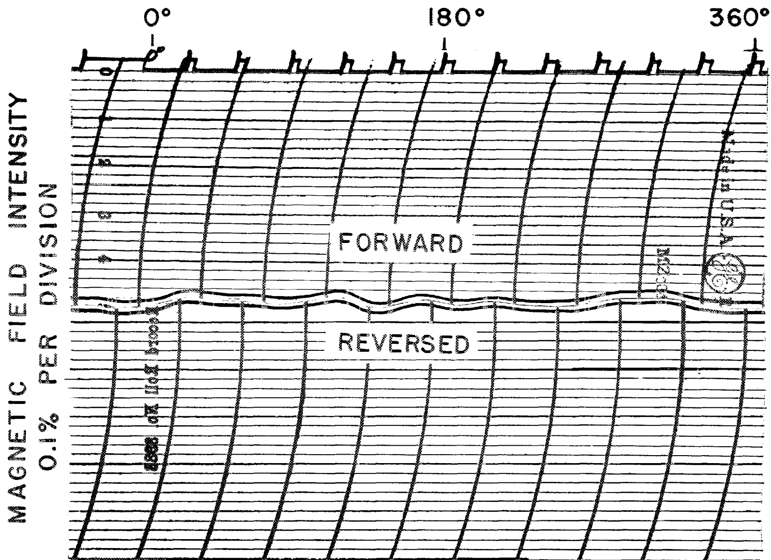
FIGURE 38. AZIMUTHAL FIELD VARIATIONS
