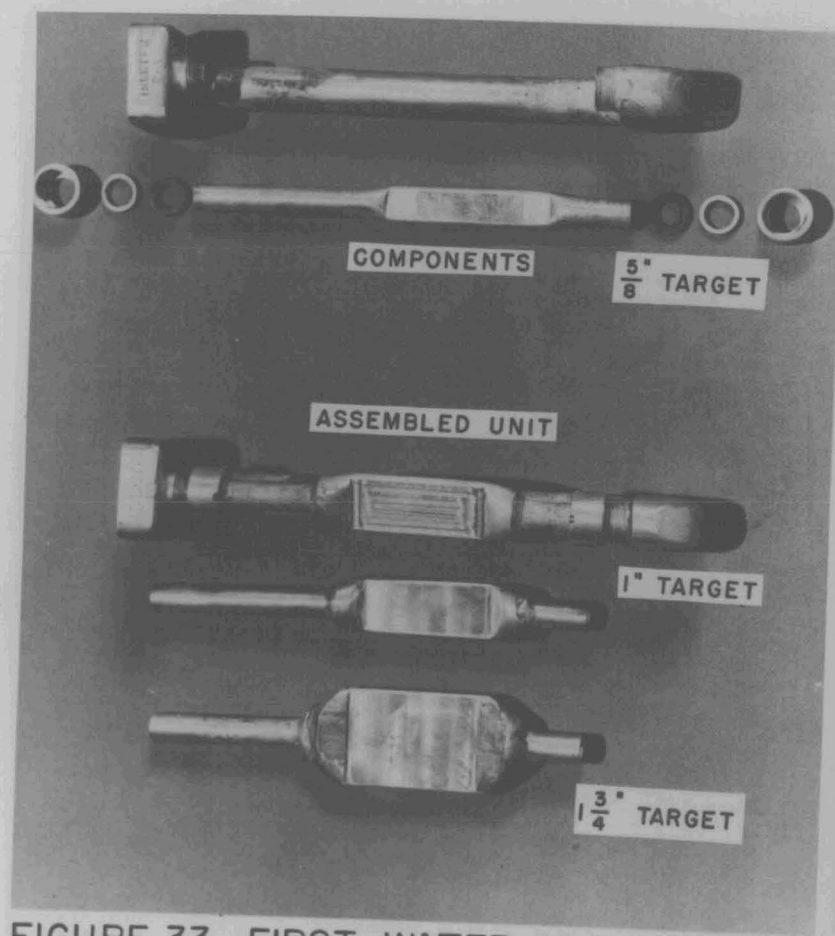
FIGURE 33. FIRST WATER-COOLING TARGET
