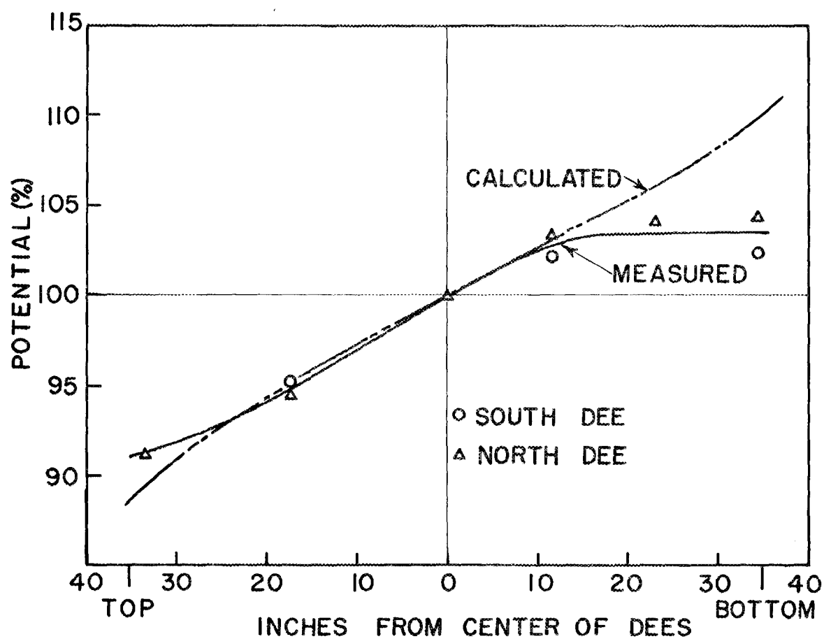
FIGURE 36. POTENTIAL DISTRIBUTION ON DEES
