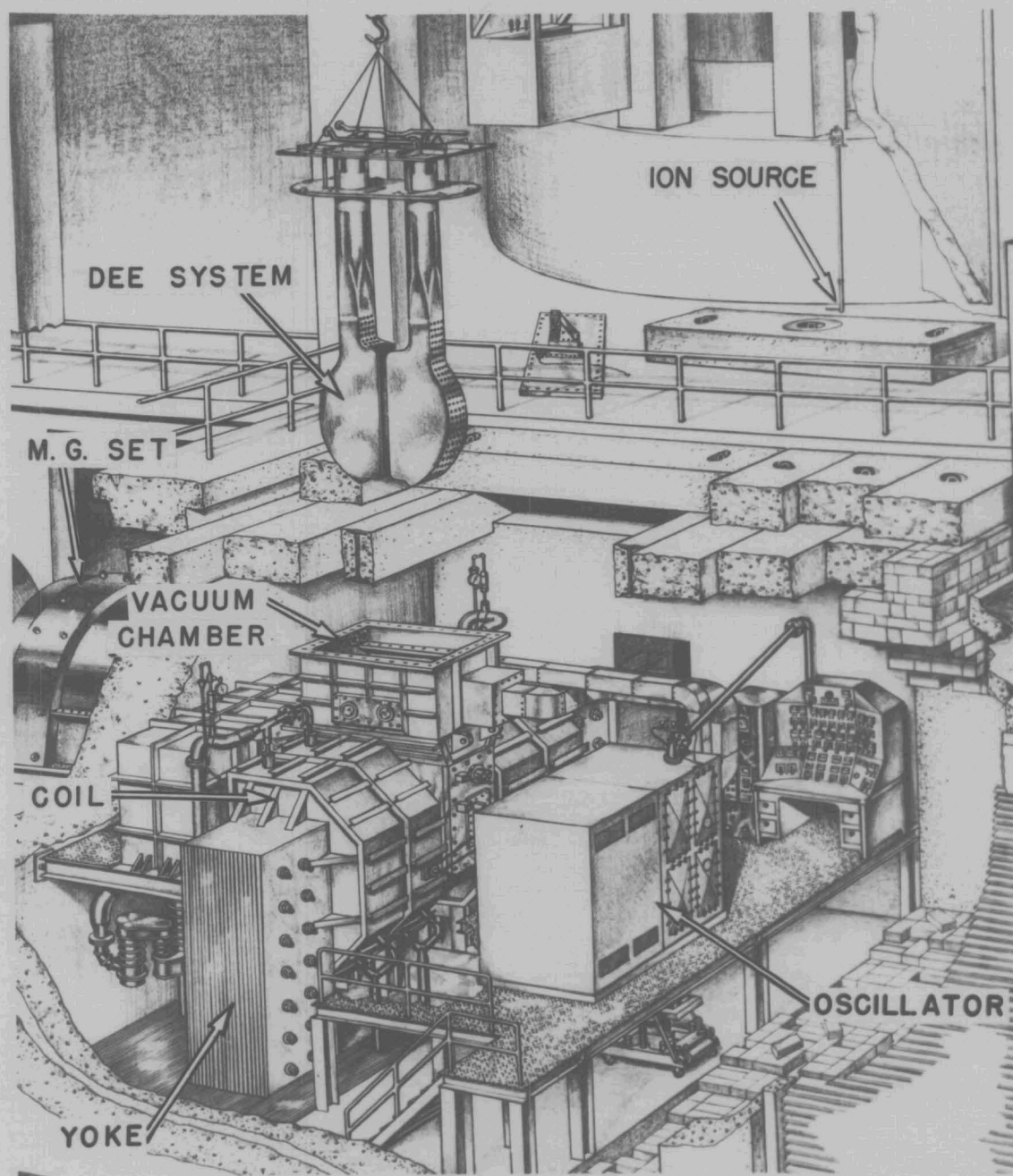
FIGURE 15. CYCLOTRON COMPONENTS
