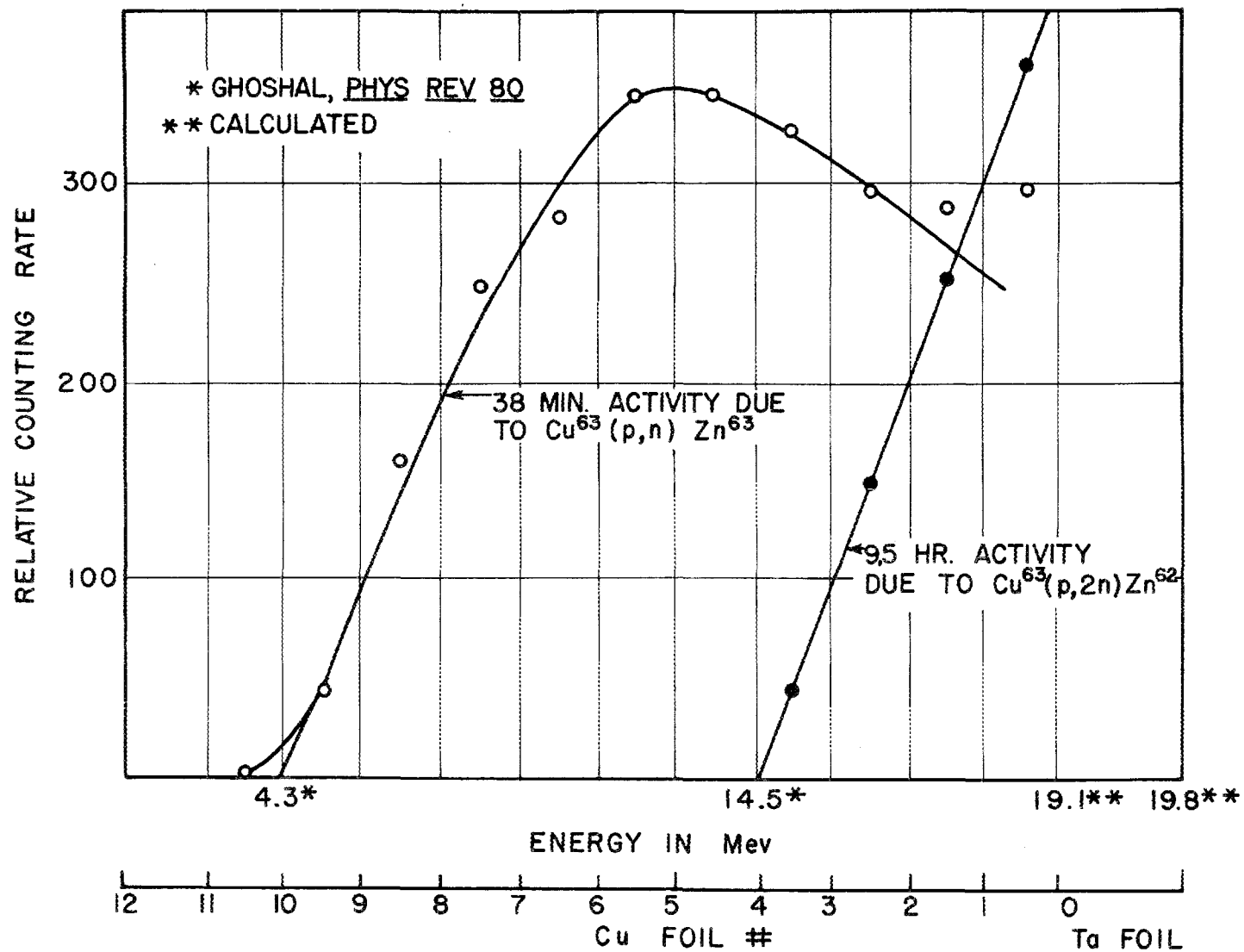
FIGURE 41. ENERGY MEASUREMENT FROM COPPER FOILS
