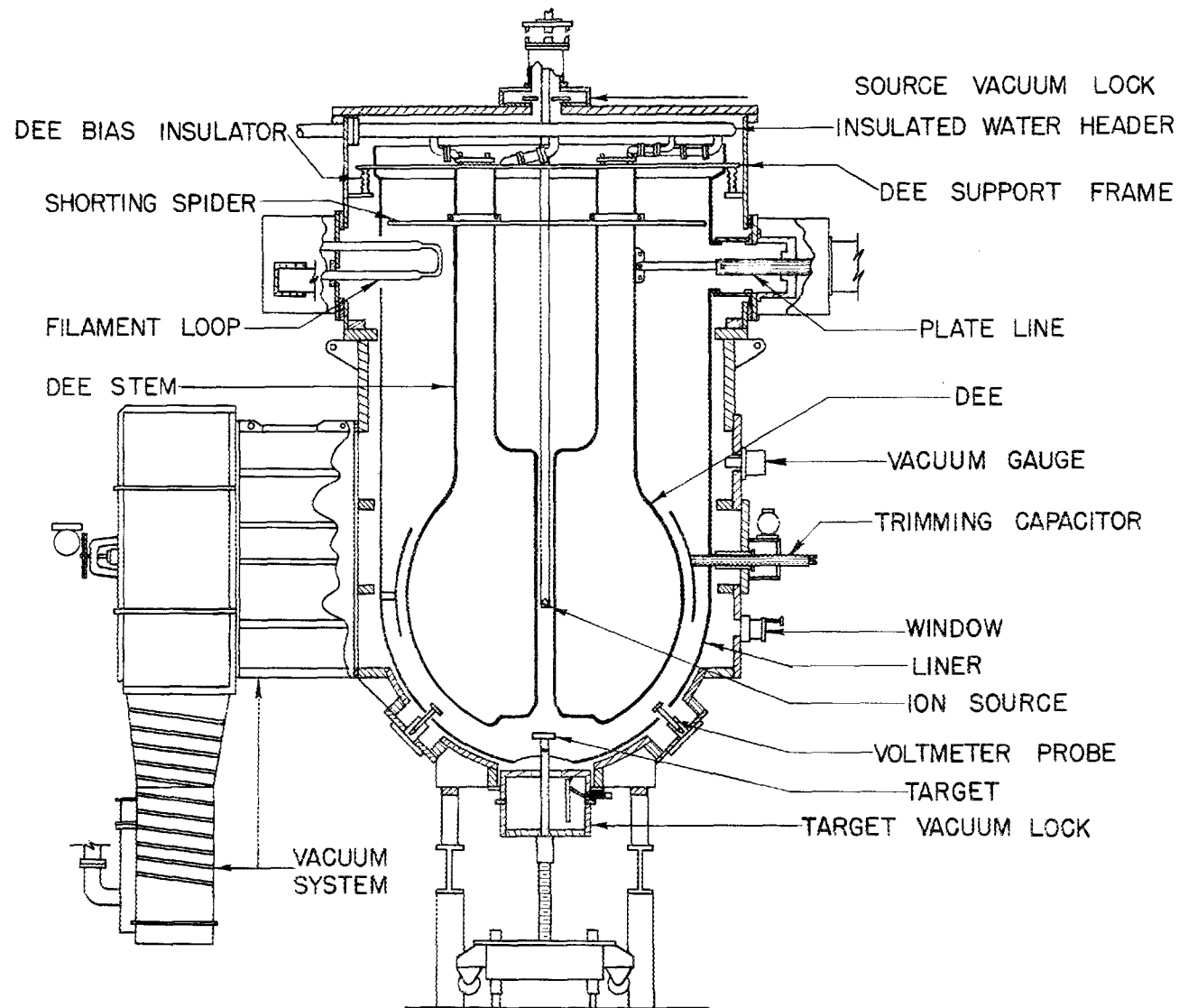
FIGURE 2. CROSS SECTION OF CYCLOTRON
