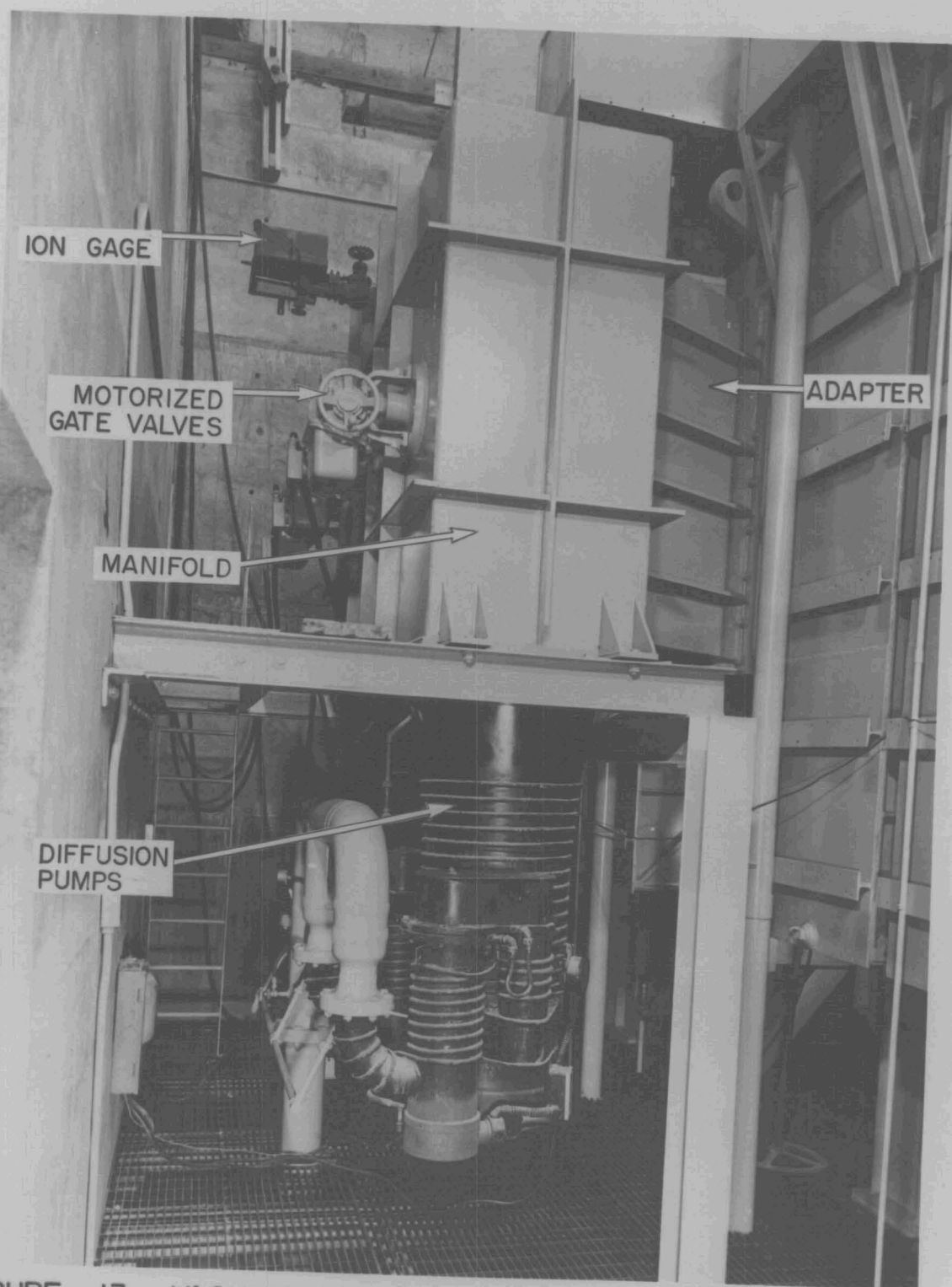
FIGURE 13 VACUUM MANIFOLD AND DIFFUSION PUMPS
