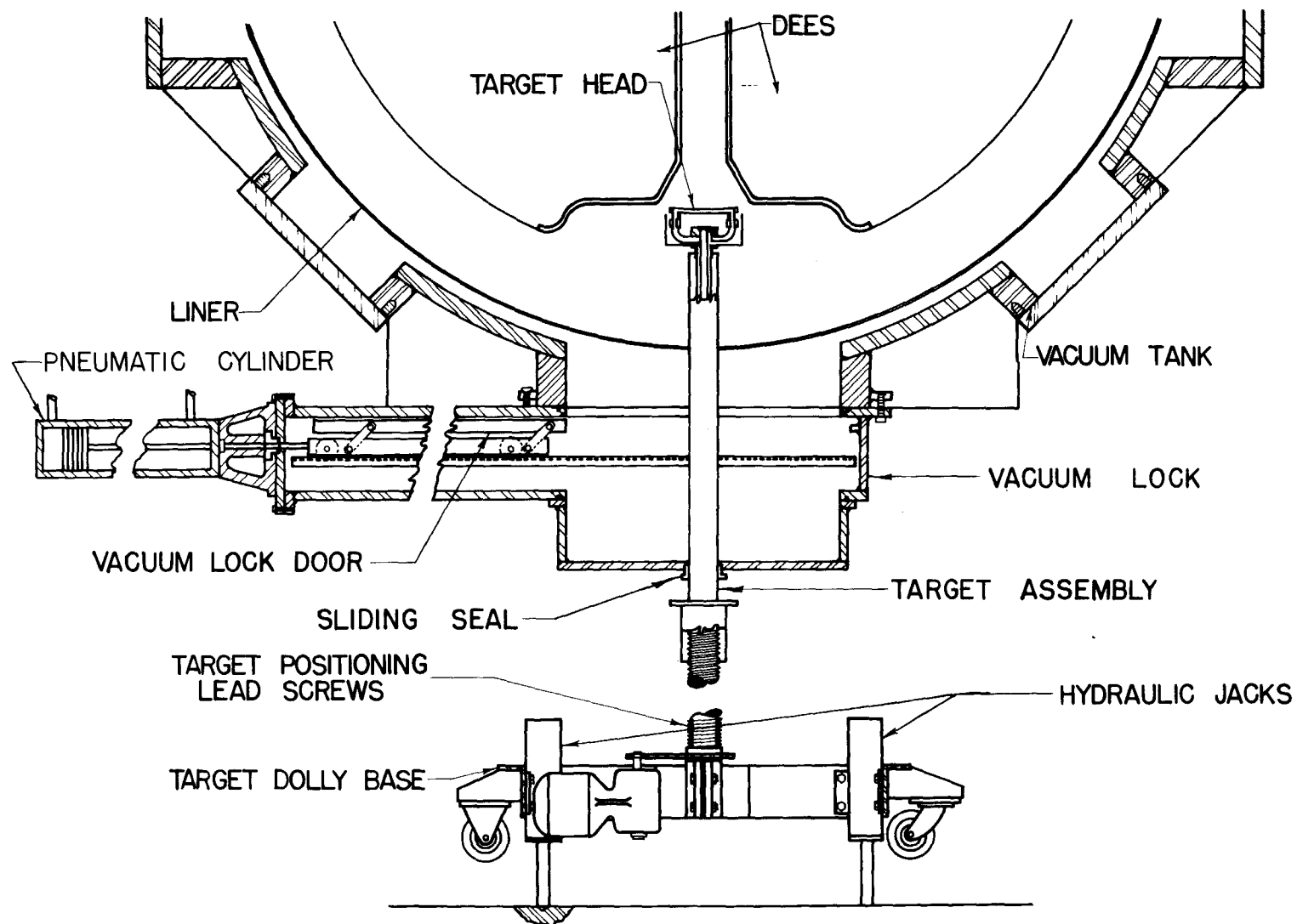
FIGURE 25 CYCLOTRON TARGET INSTALLATION
