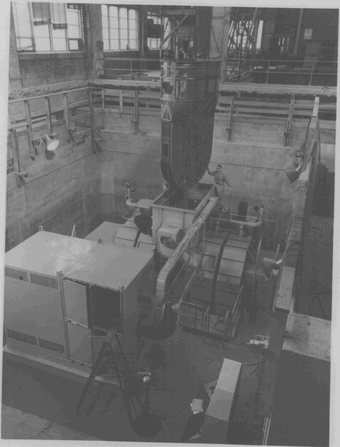
FIGURE 18. INSTALLING LINER
