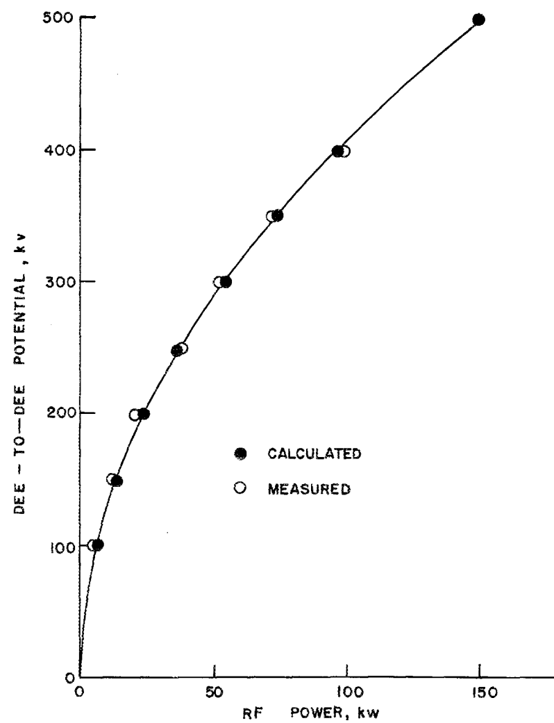
FIGURE 5. POWER FOR DEE EXCITATION
