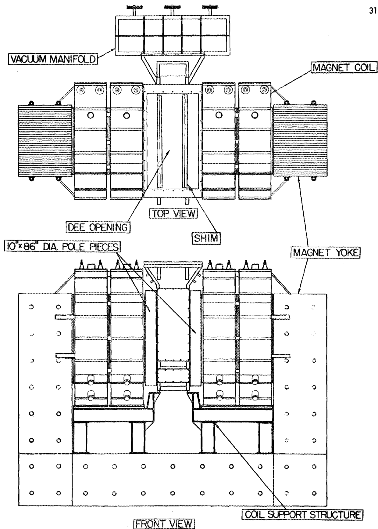
FIGURE 7. 86 INCH MAGNET, SKETCH
