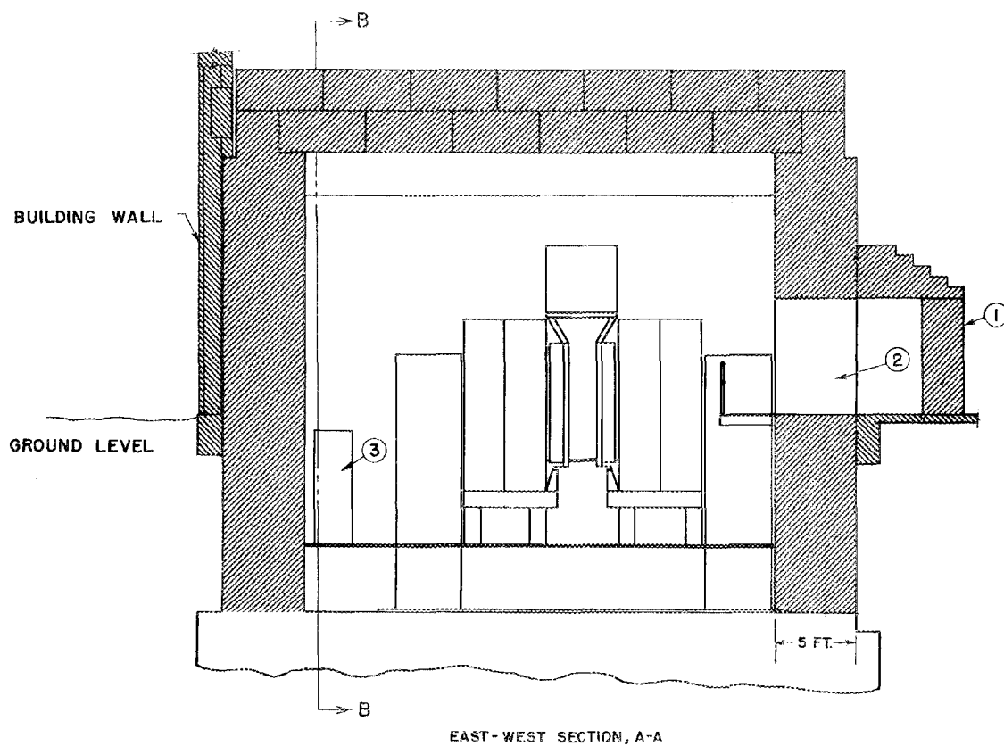
FIGURE 31. CYCLOTRON SHIELDING
