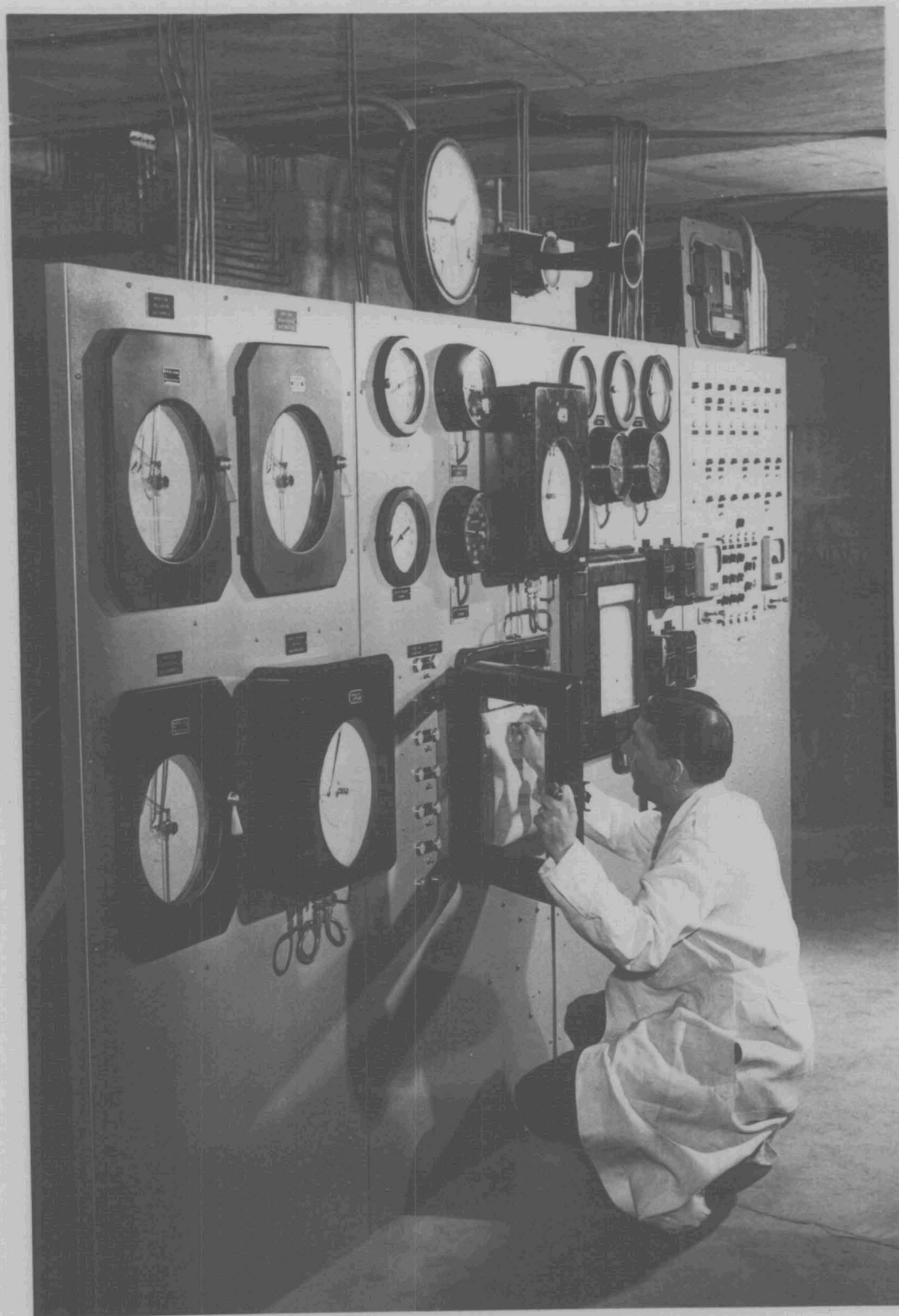
FIGURE 32. UTILITIES PANEL
