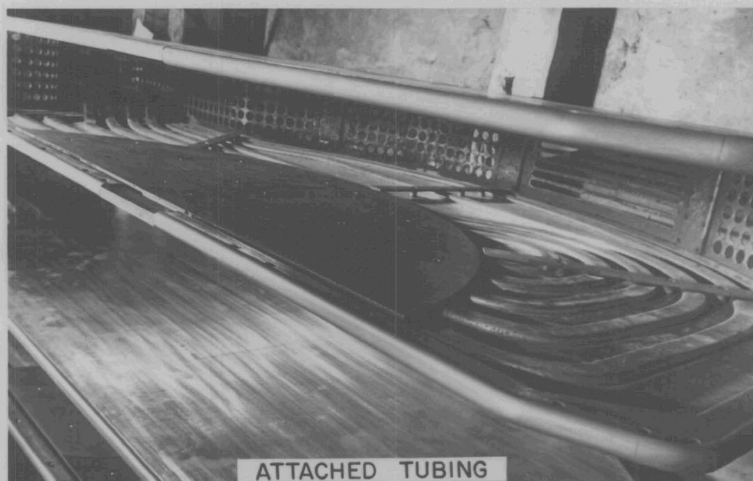
FIGURE 16. WATER COOLING OF DEES
