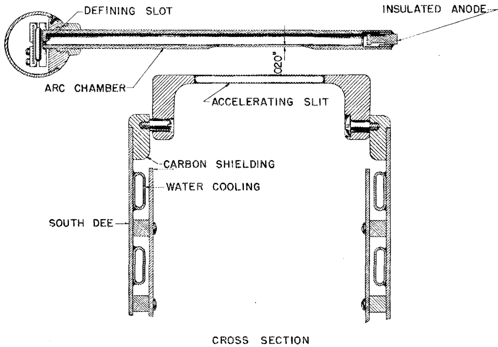
FIGURE 22. ION SOURCE
