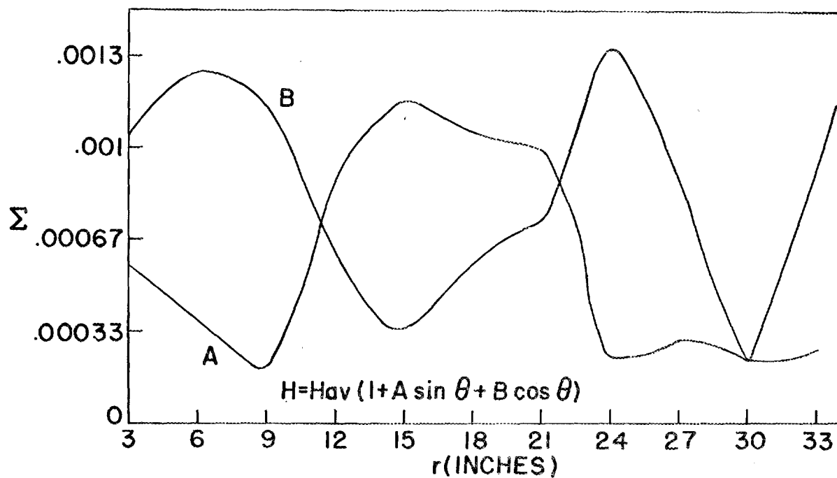
FIGURE 35. HARMONIC ANALYSIS OF MAGNETIC FIELD
