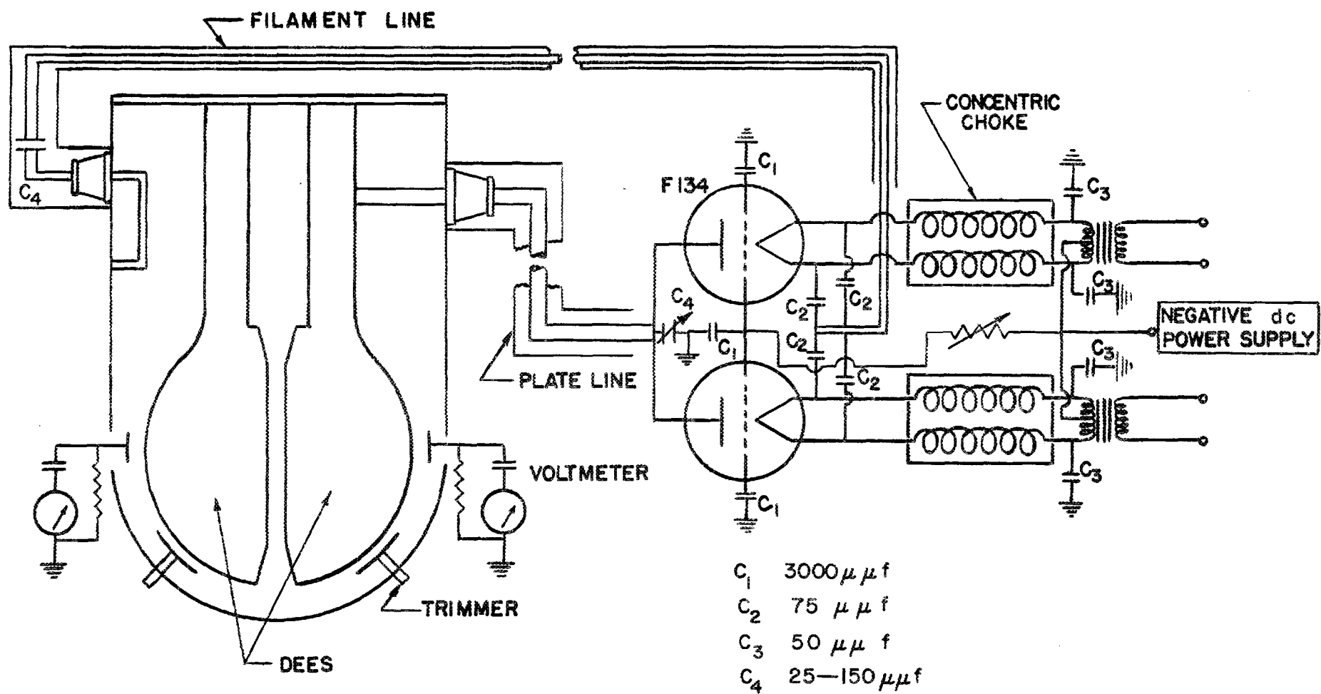
FIGURE 39. RF SYSTEM, ORIGINAL INSTALLATION
