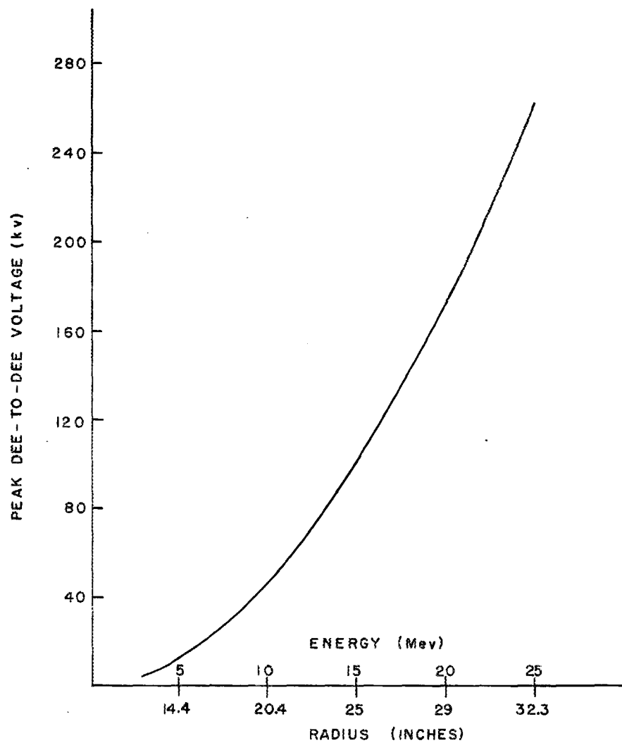
FIGURE 4. THRESHOLD VOLTAGE
