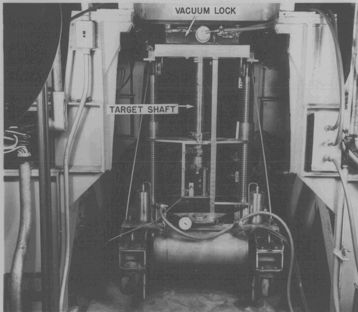
FIGURE 24. TARGET DOLLY
