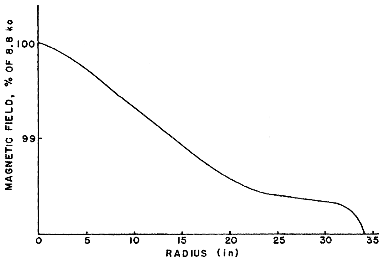
FIGURE 10. MAGNET CHARACTERISTICS
