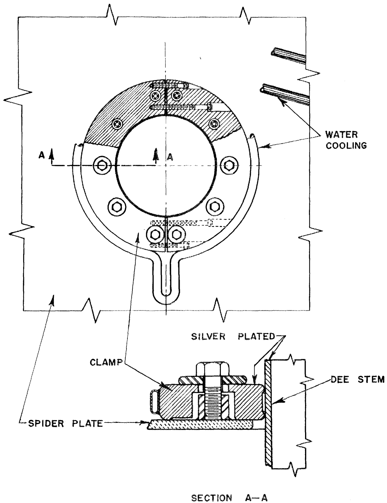
FIGURE 17. RF JOINT AT SPIDER
