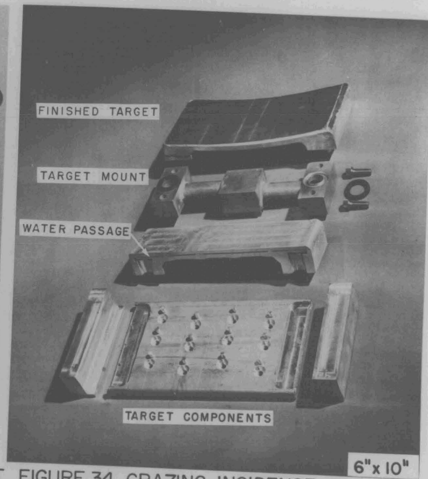
FIGURE 34. GRAZING INCIDENCE TARGET
