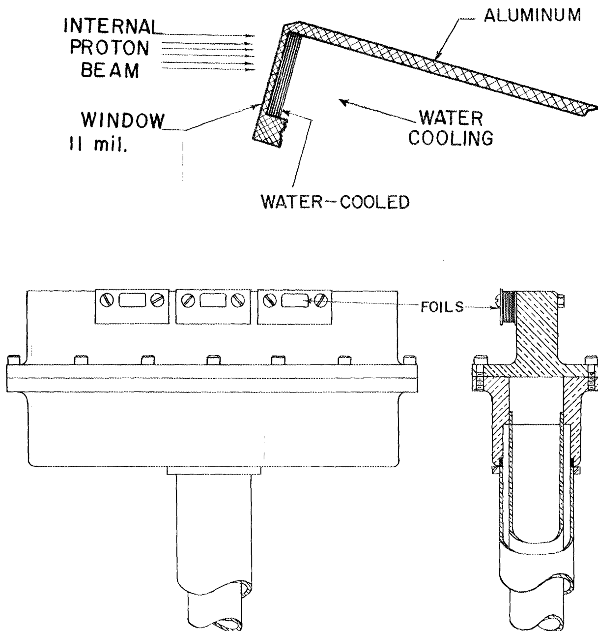
FIGURE 27. EXPERIMENTAL TARGETS
