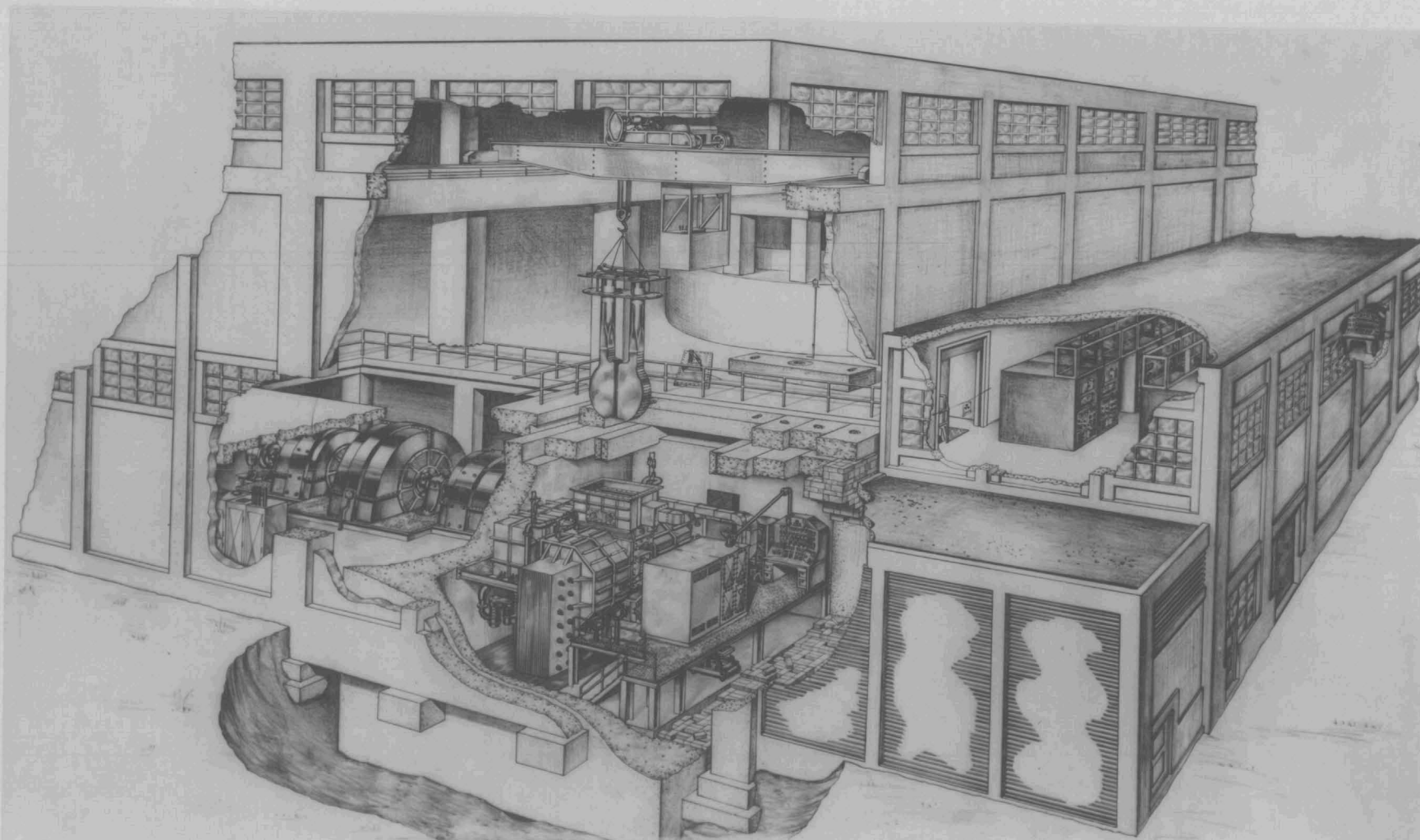
FIGURE 1 THE 86 INCH CYCLOTRON INSTALLATION
